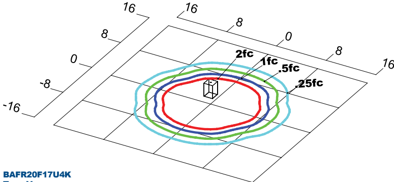
BAFR20F17U4K Type V Grid in feet, Mounting Height = 3.5 ft.
