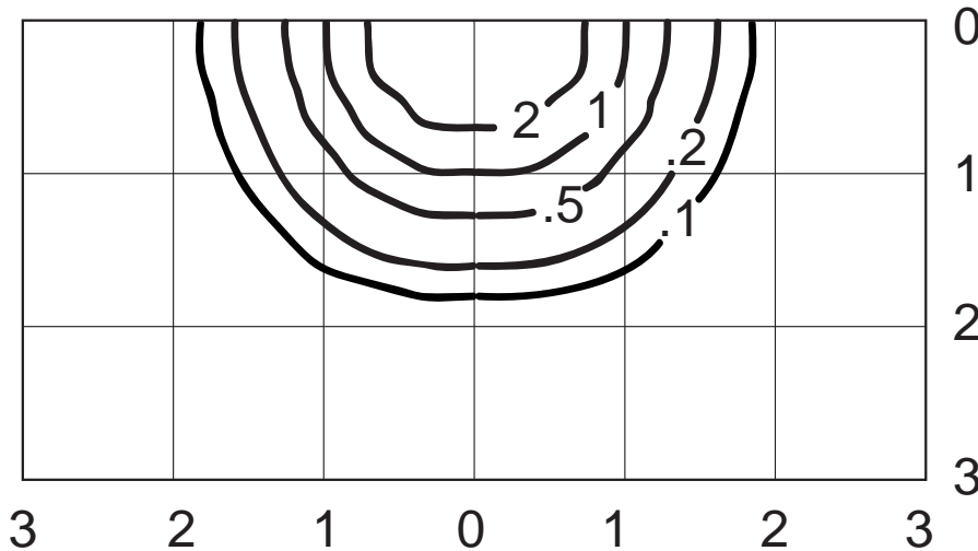
W60F84 - 84W Compact Fluorescent - Downlight Portion only
